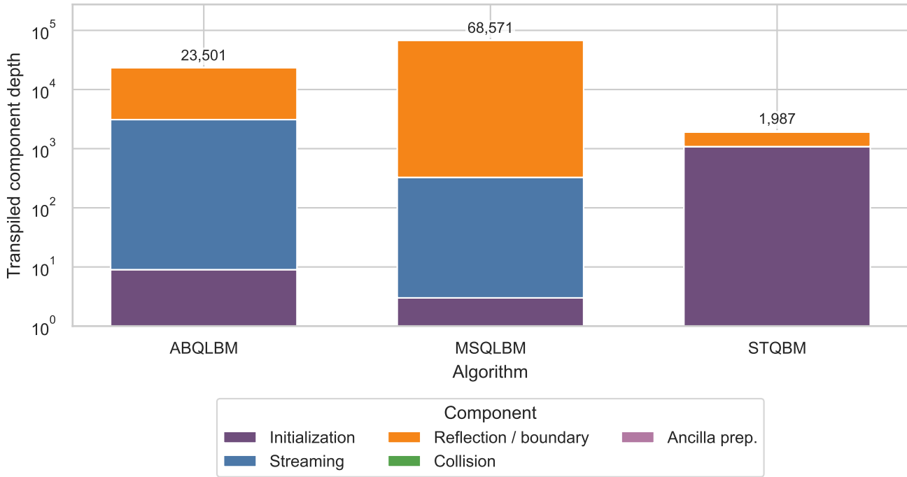
8x8 lattice, 2 bounce-back obstacles
