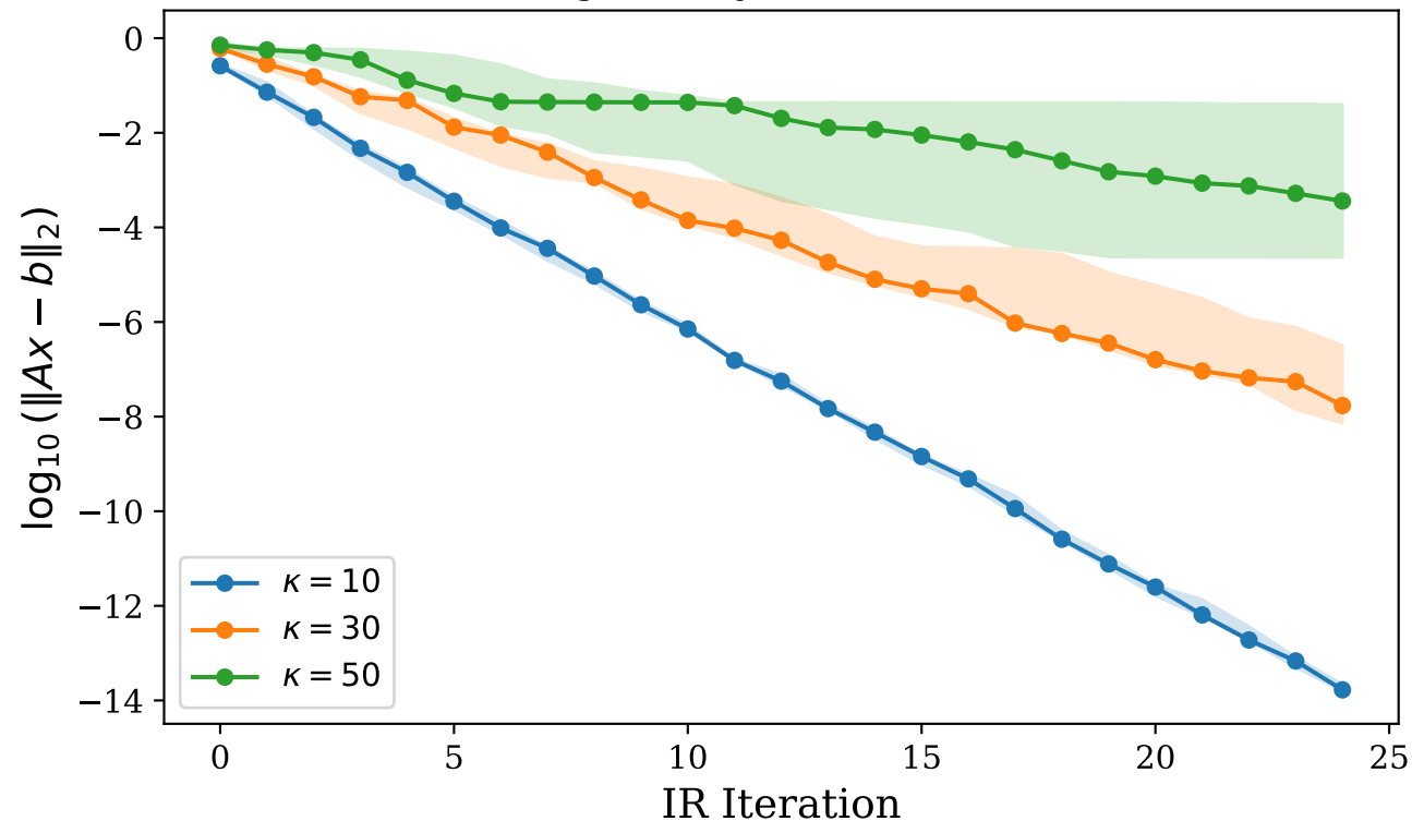
Residual Convergence by Condition Number ( n = 16 )
