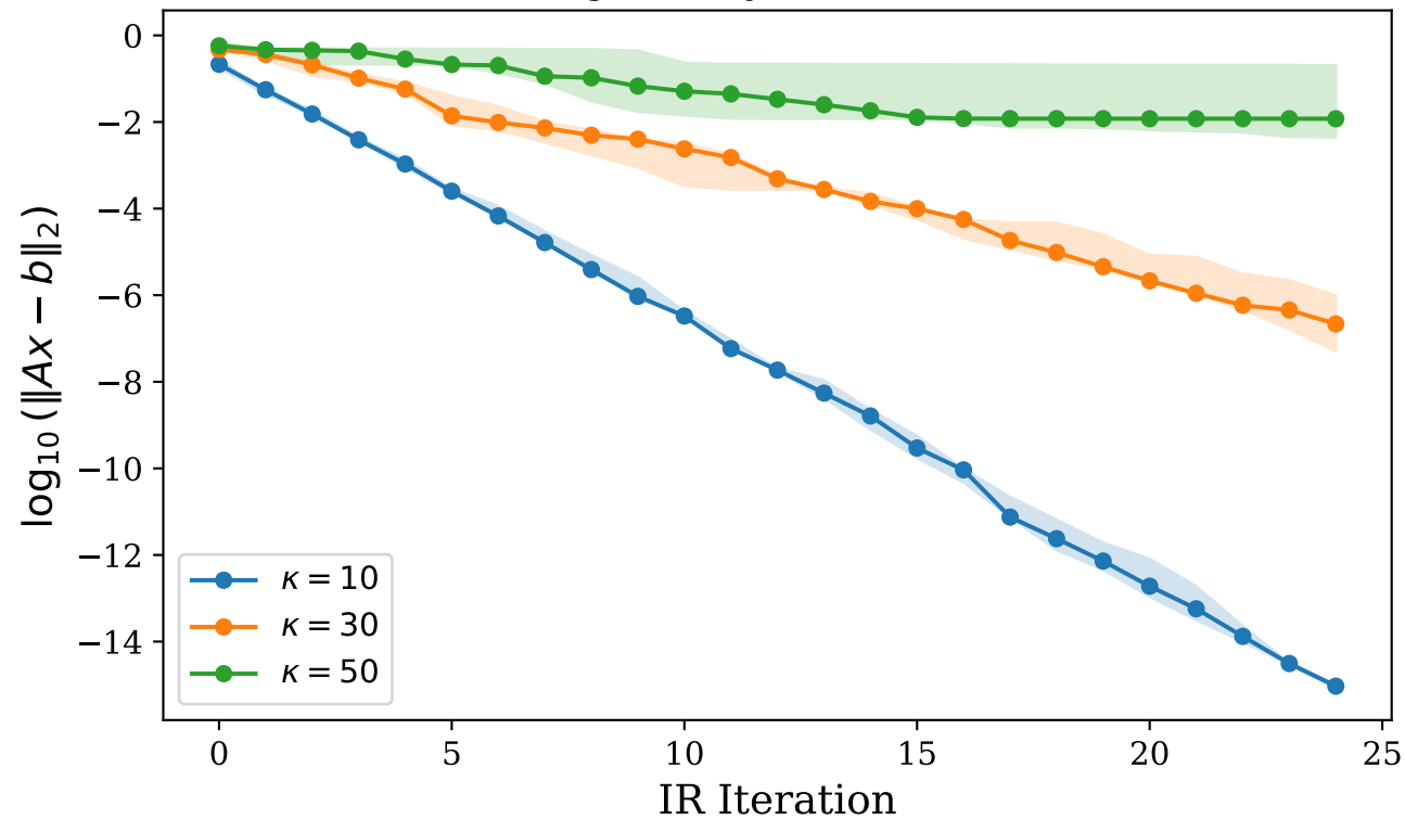
Residual Convergence by Condition Number ( n = 8 )
