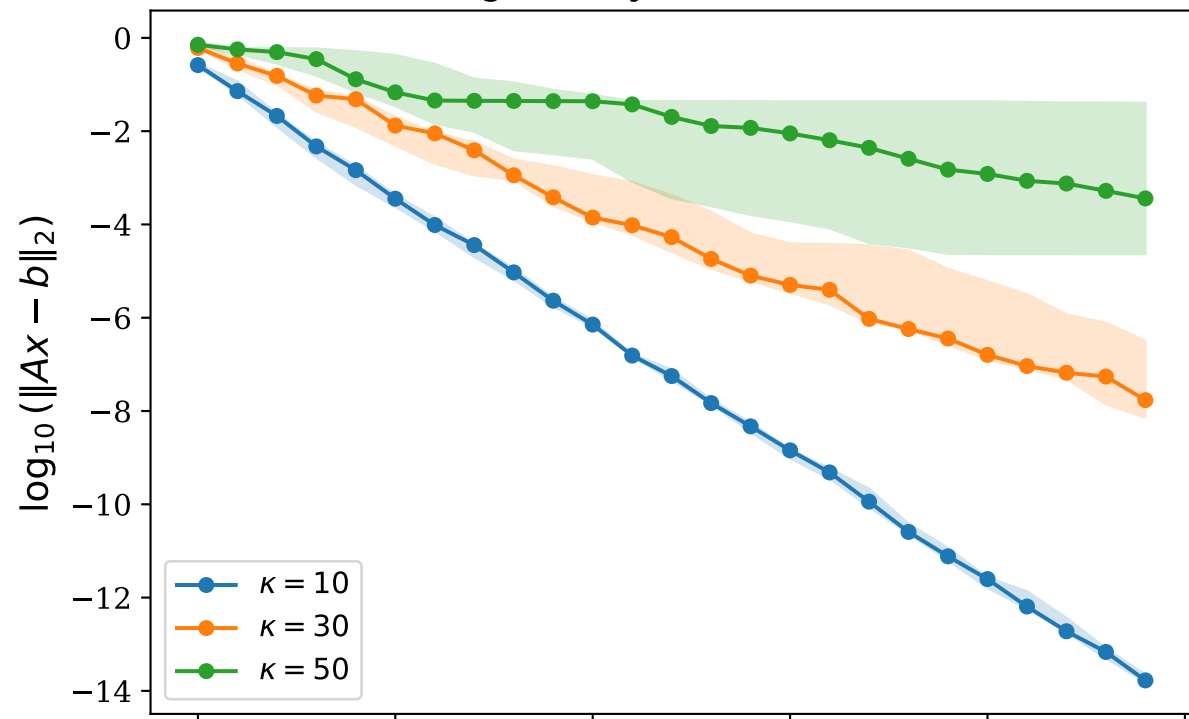
Residual Convergence by Condition Number ( n = 16 )
