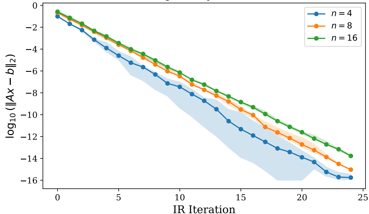
Residual Convergence by Problem Size ( \kappa = 10 )
