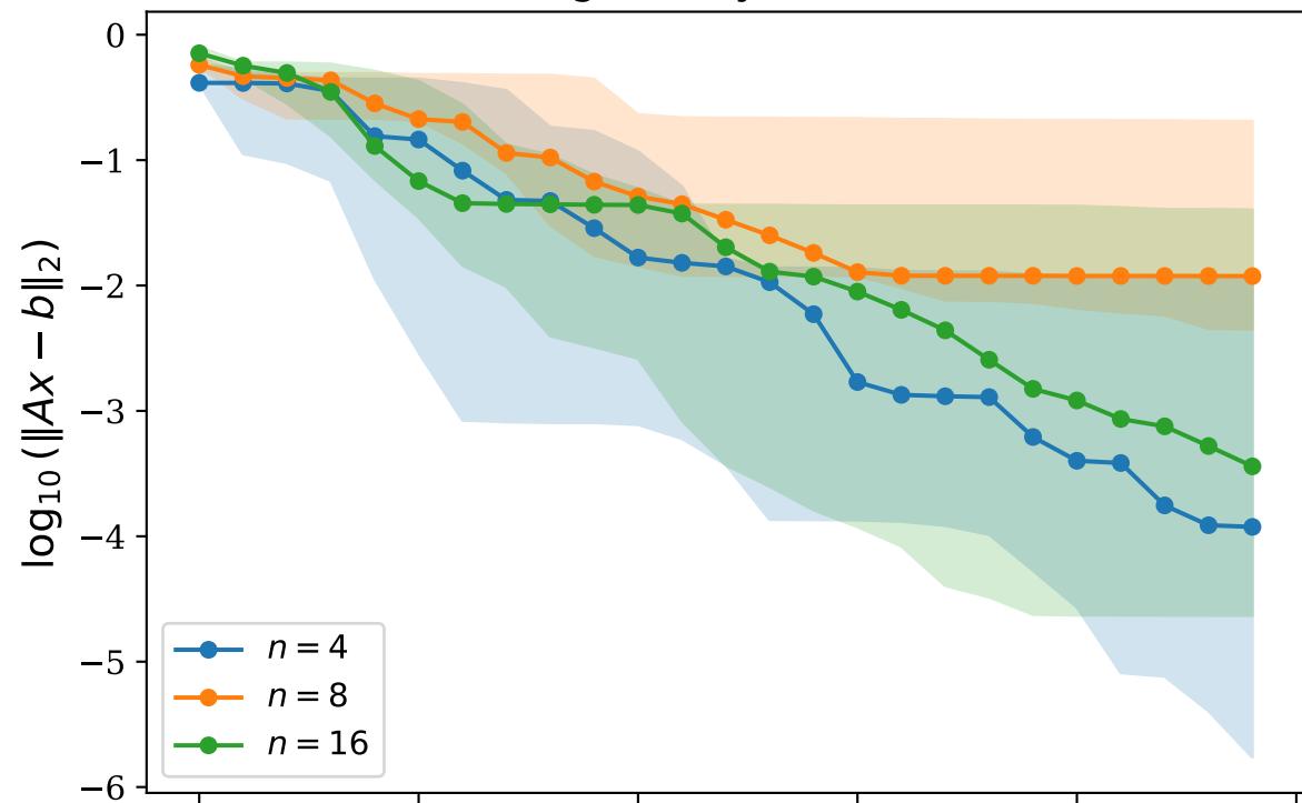
Residual Convergence by Problem Size ( \kappa = 50 )
