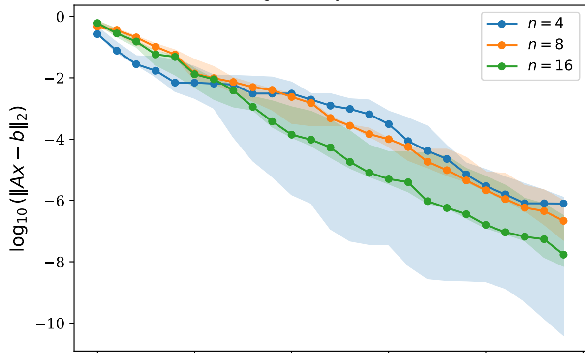
Residual Convergence by Problem Size ( \kappa = 30 )
