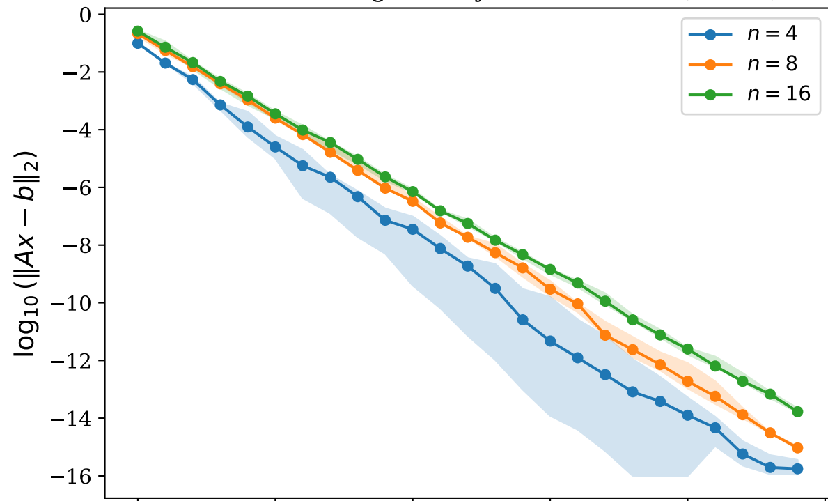
Residual Convergence by Problem Size ( \kappa = 10 )
