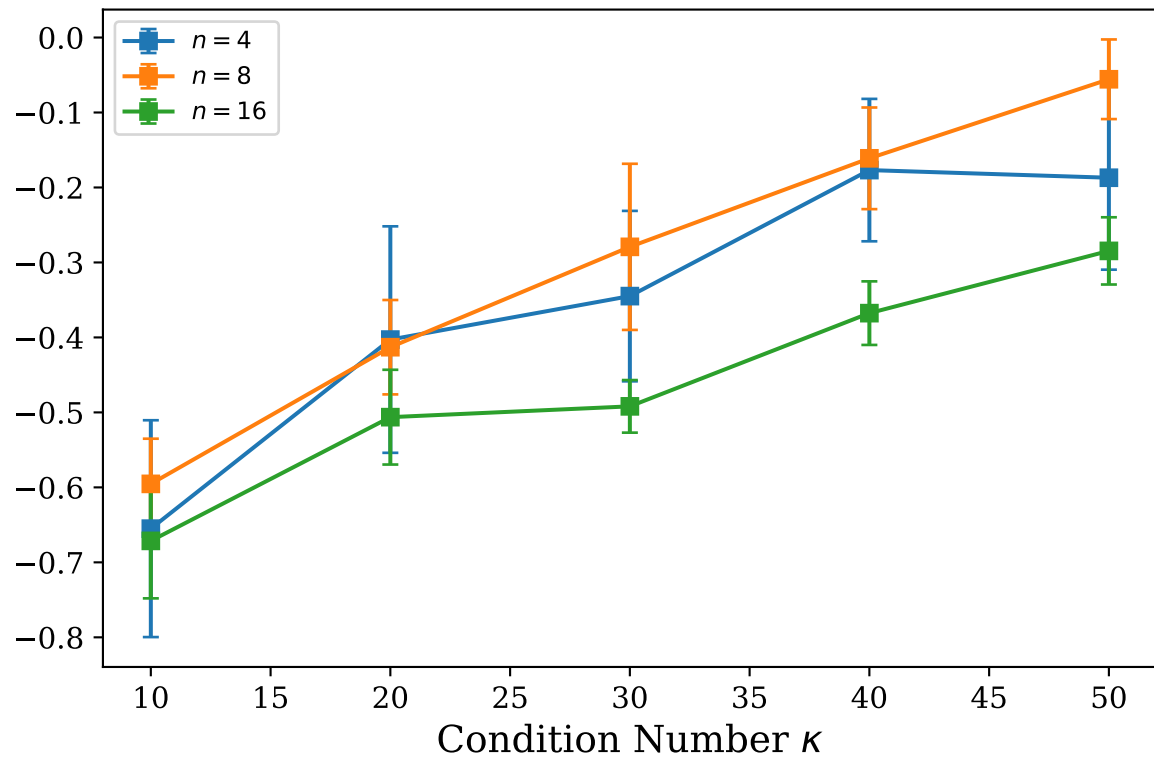
Rate vs. Condition Number
