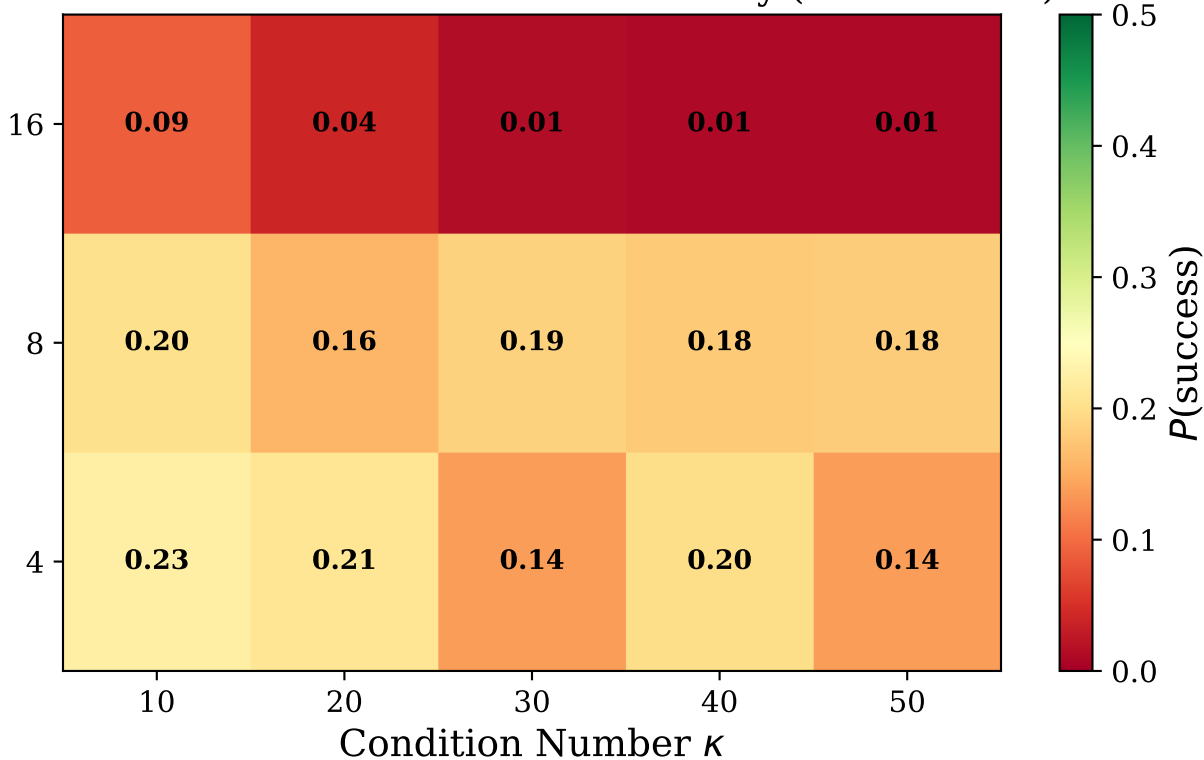
Mean Post-Selection Success Probability (over 5 seeds)
