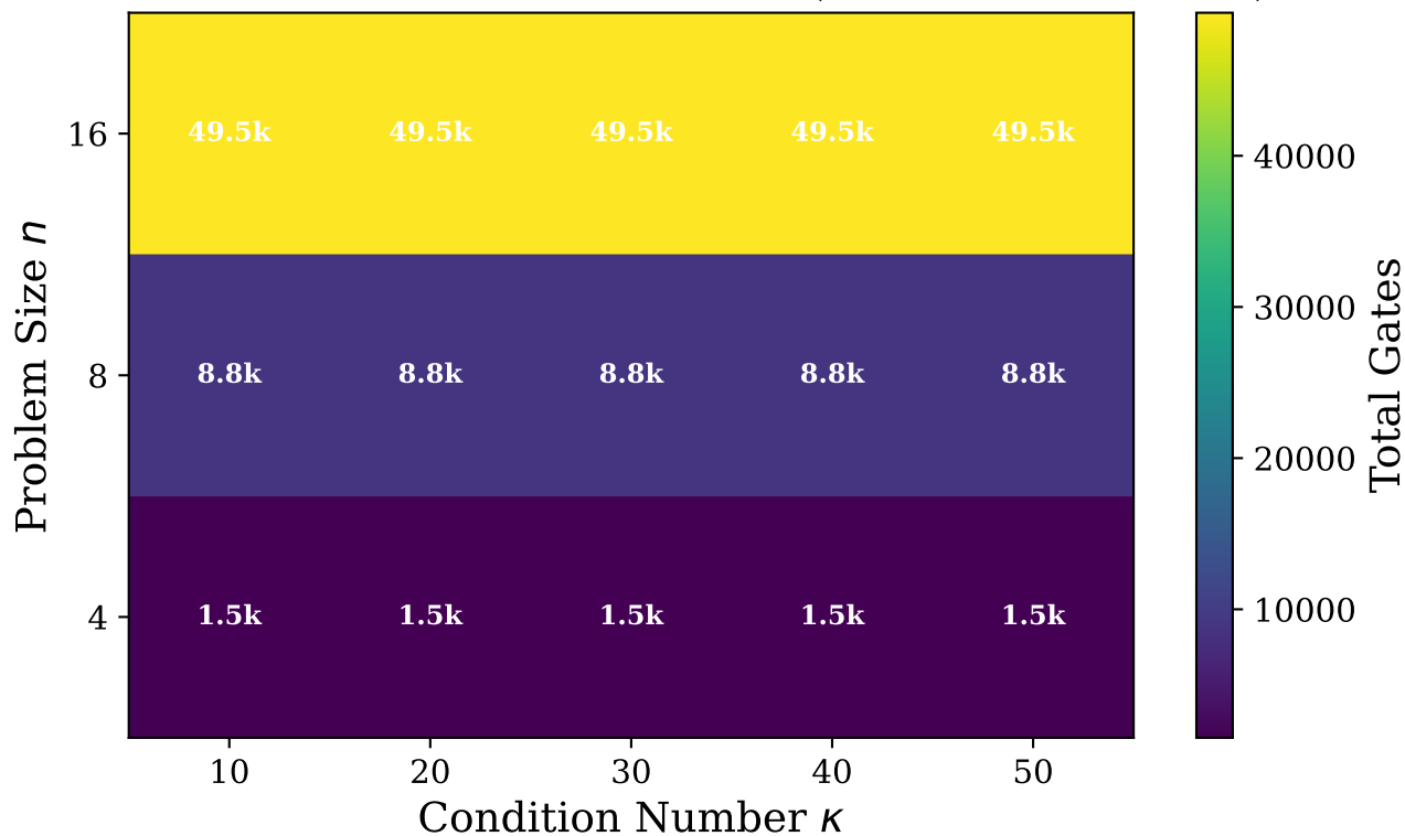
Total Gate Count over 20 IR Iterations (median over 5 seeds)
