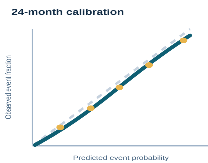
Figure 3 · Calibration and coefficient-sign stability
