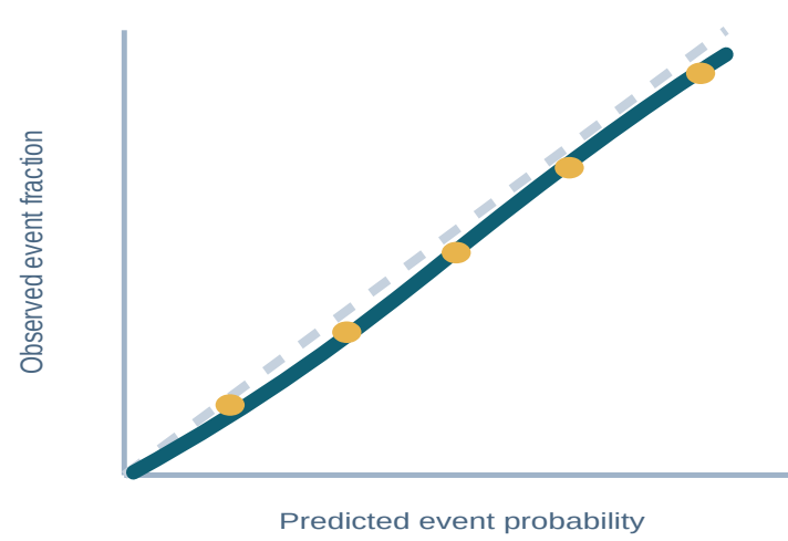
Figure 3 · Calibration and coefficient-sign stability
