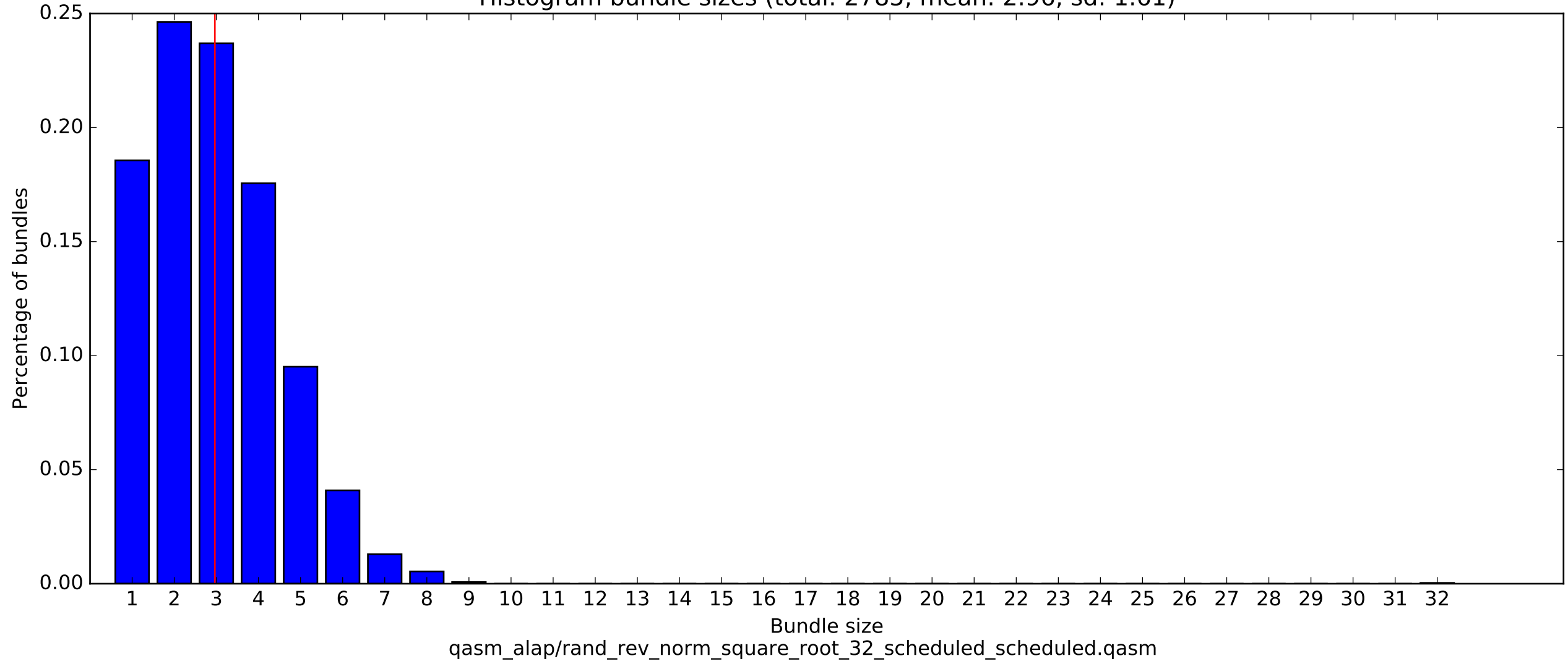
Histogram bundle sizes (total: 2785, mean: 2.96, sd: 1.61)
