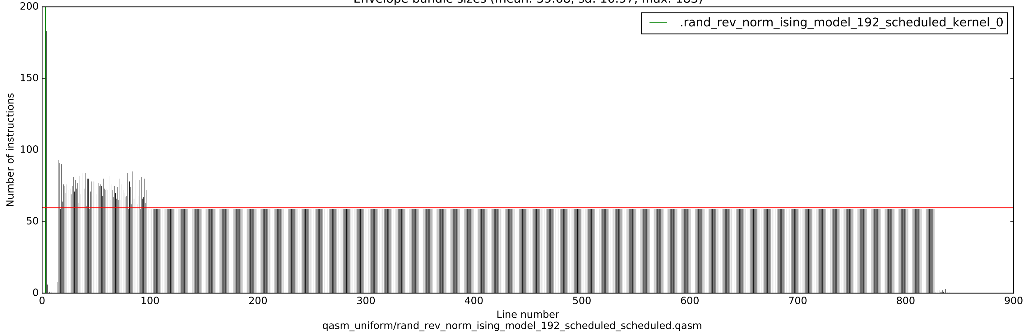
Envelope bundle sizes (mean: 59.68, sd: 10.97, max: 183)
