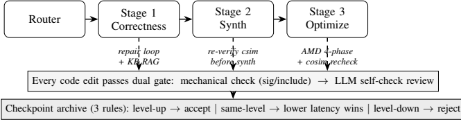
Fig. 1: Agent architecture. Three stages run sequentially; every code edit (in any stage) passes a dual review gate before the checkpoint arbitrates whether it enters the archive. The checkpoint’s monotone-level rule gives automatic rollback—a failed candidate simply never replaces the best.
