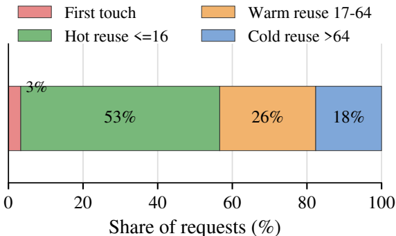
(a) Shared replay adapter churn
