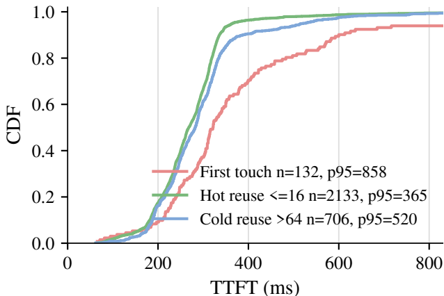
(b) S-LoRA TTFT by reuse distance
