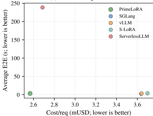
(a) Cost--latency Pareto view
