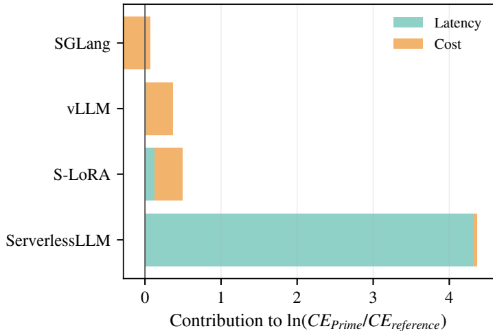
(b) CE log-contribution audit
