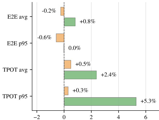
Improvement vs NVMe-pre (%) (b) End-to-end and decode impact
