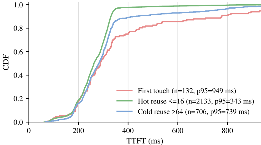
(b) S-LoRA TTFT by reuse distance
