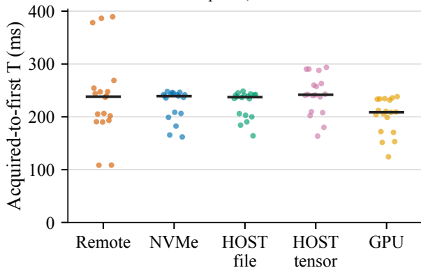
(b) Acquired-to-first token
