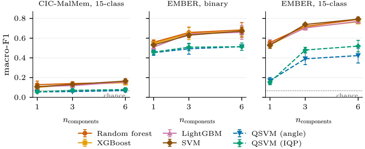
Figure 1: Macro-F1 against the shared feature/qubit budget; solid lines are classical, dashed the QSV encodings. The gap on EMBER binary widens with n_c — the QSV gains 0.055 from one to six components where the random forest gains 0.125. CIC binary is absent; see §4.
