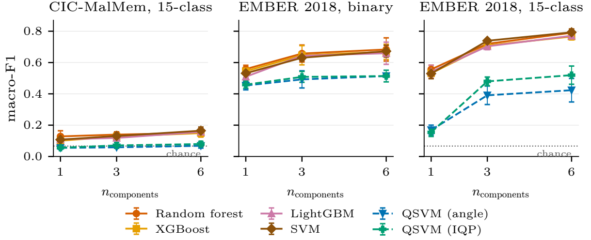
Figure 1: Held-out macro-F1 against the shared feature/qubit budget. Solid lines are classical models, dashed lines the QSV encodings; error bars are one standard deviation across the five outer folds. CIC binary is absent because no sweep of it can be grouped (§5). Note that the classical-quantum gap on EMBER binary widens with n_{\text{components}} : the QSV gains 0.055 macro-F1 from one to six components where the random forest gains 0.125.
