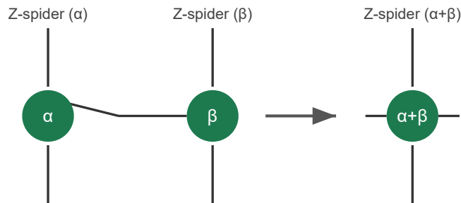
Figure 1. Spider fusion: two connected Z-spiders merge into one, preserving the linear map.
