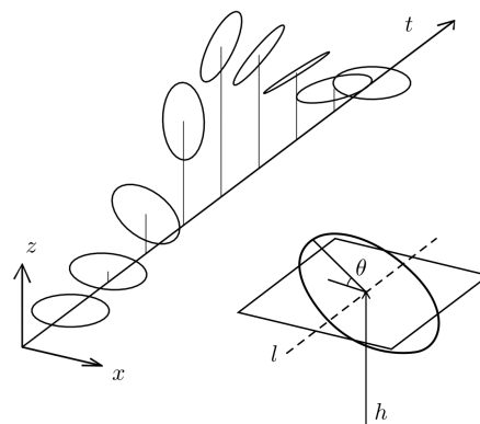
Figure 1: The pancake at different t during a 1-toss. \theta is the rotation about the flipping axis \ell ( \ddot{\theta} = \alpha for t < t_0 ), and h the CM height ( \ddot{h} = a for t < t_0 ).
