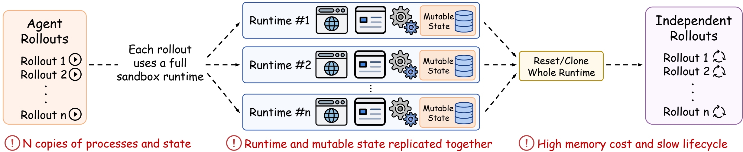
(a) Conventional Sandboxes
