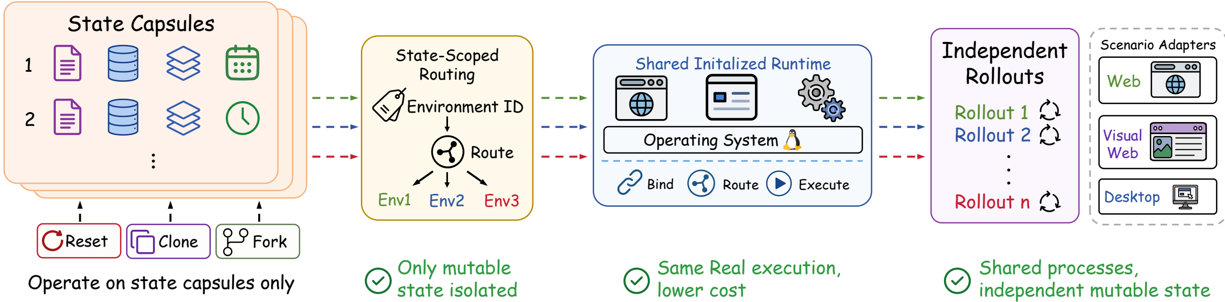
(b) CUA-Sandbox via Runtime-State Separation
