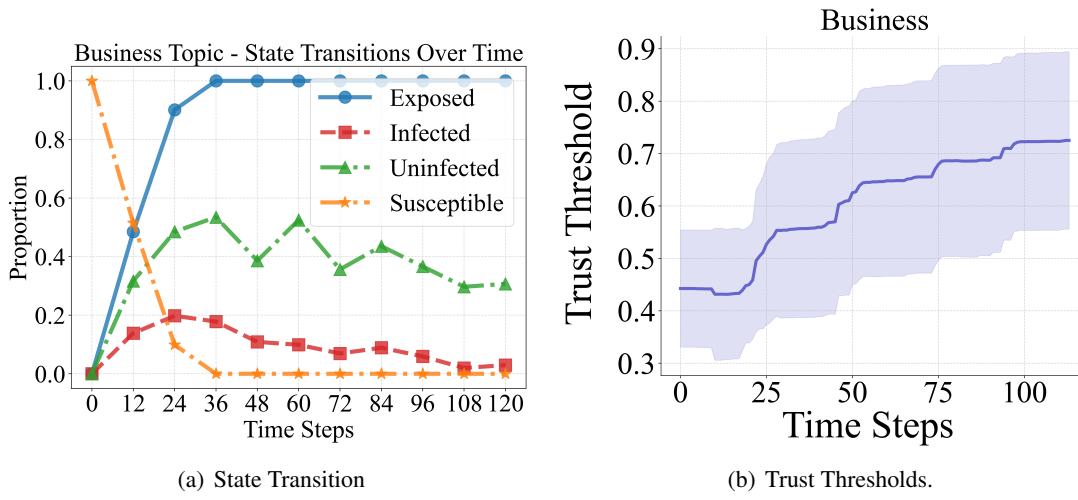
Figure 17: Long-Term dynamics of User States and Trust Thresholds
