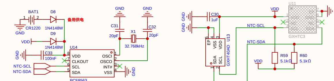
RTC实时时钟
