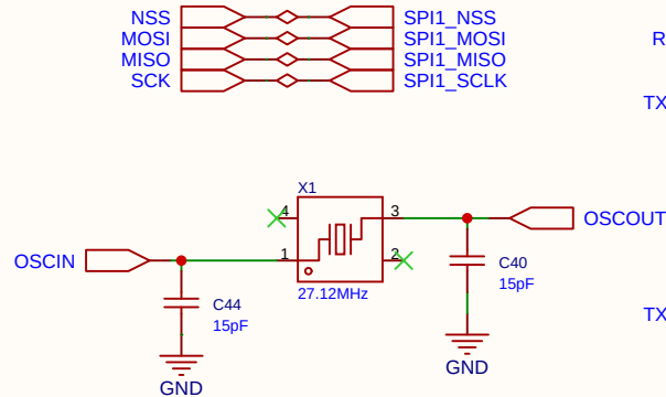
RC522晶振
