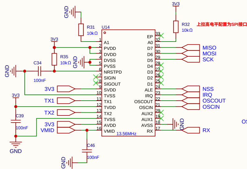
RFID_RC522读写芯片
