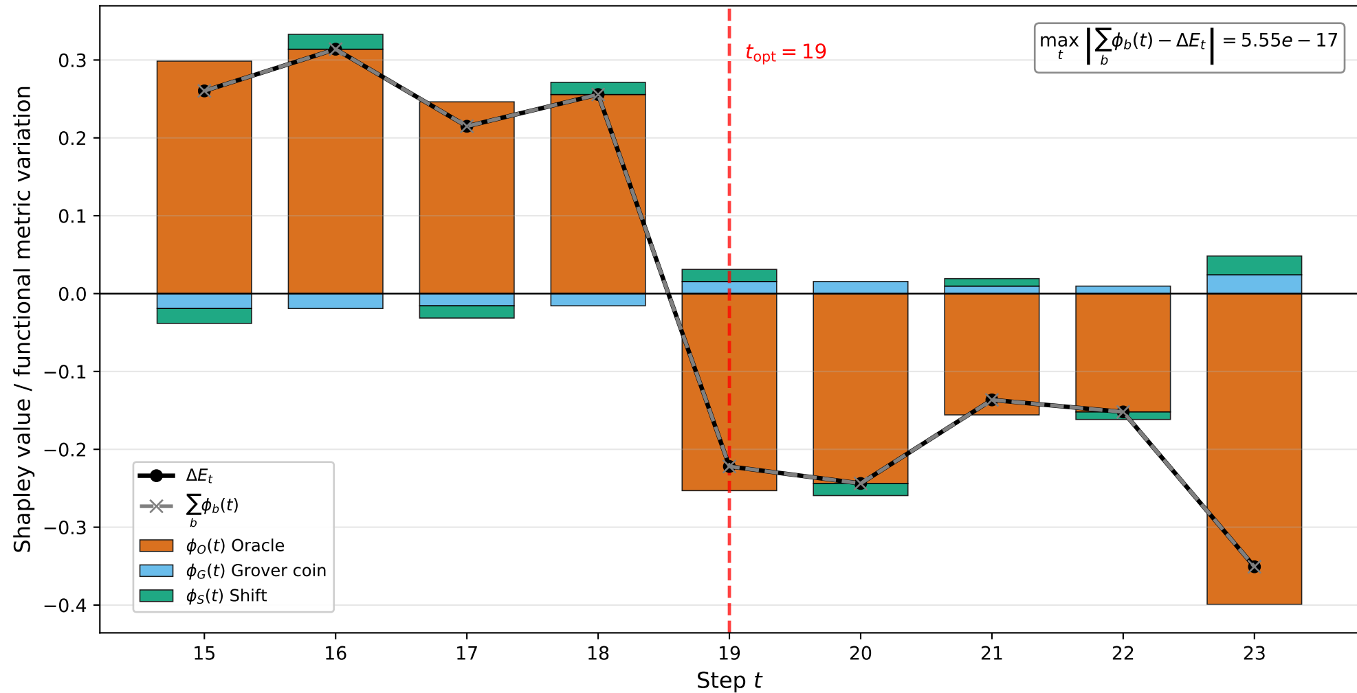
QSMEF: Shapley profile | correct implementation
