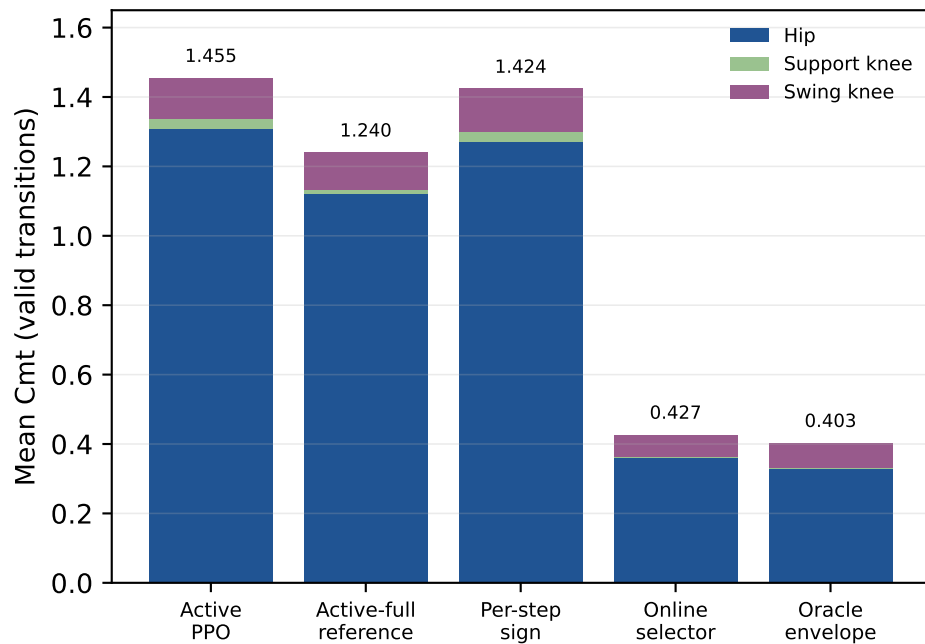
c Selector lowers actuator Cmt
