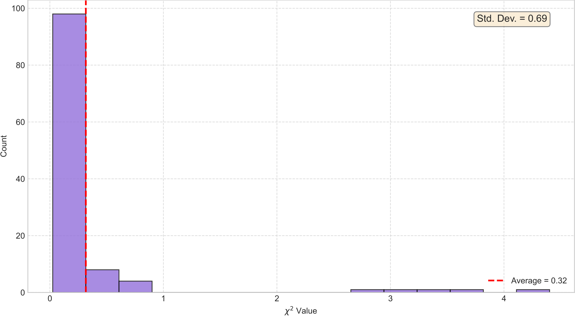
Chi-Squared ( \chi^2 ) Distribution of Fits
