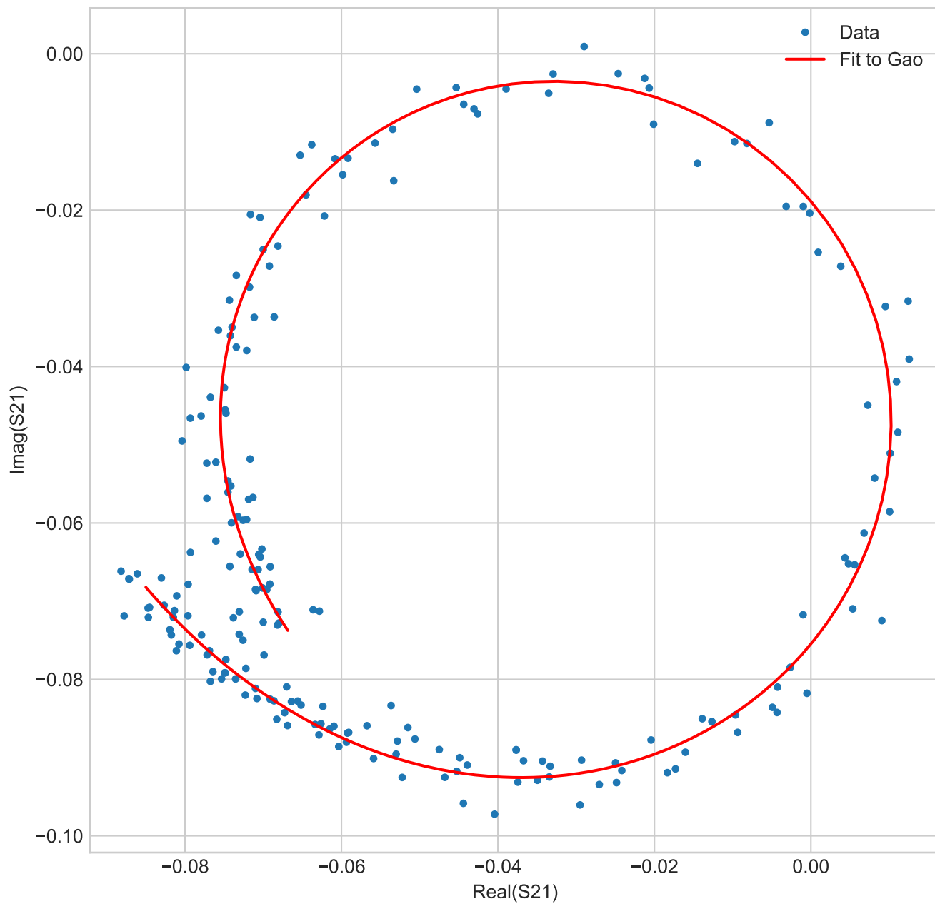
Refined Resonance Circle Fit
