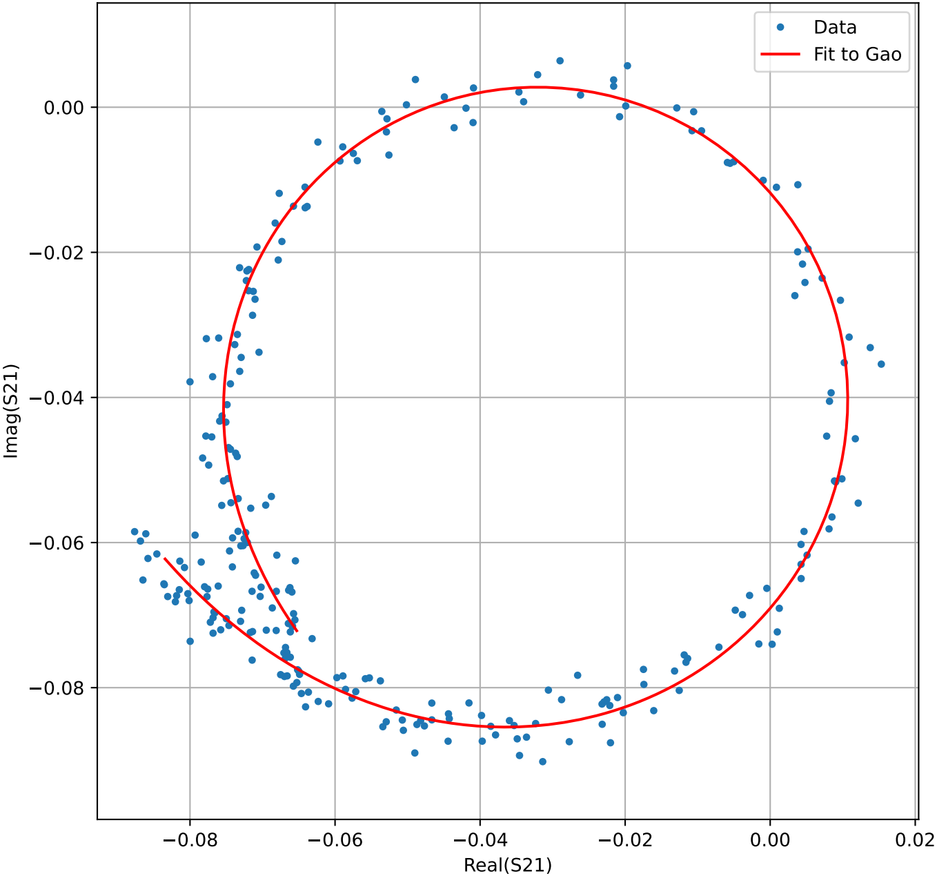
Refined Resonance Circle Fit
