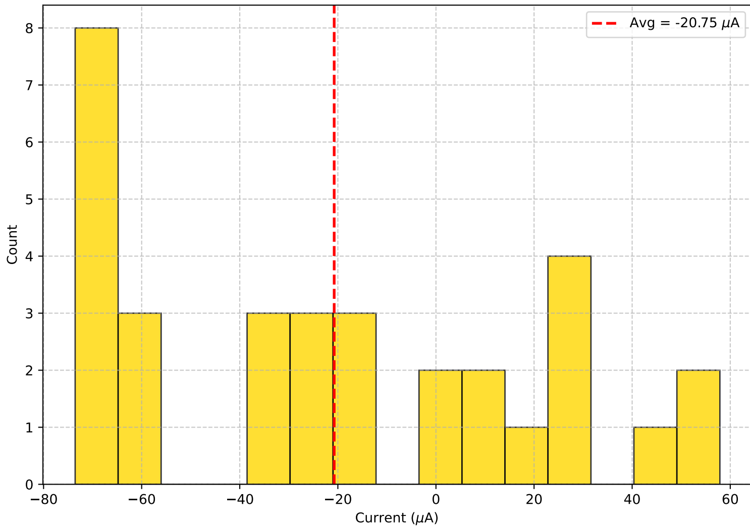
Offset Current ( I_0 ) Distribution
