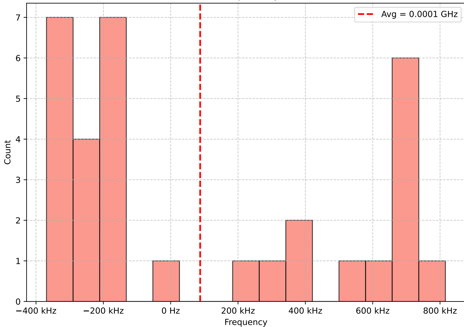
Base Resonator Frequency ( f_b ) Distribution
