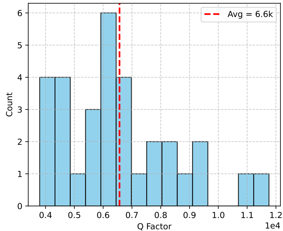
Coupling Q ( Q_c )
