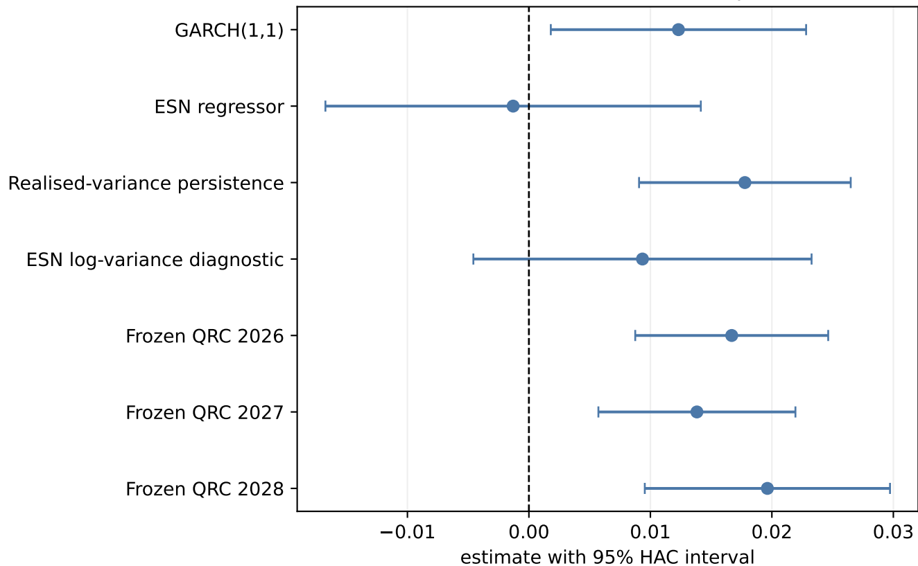
Mincer-Zarnowitz intercept
