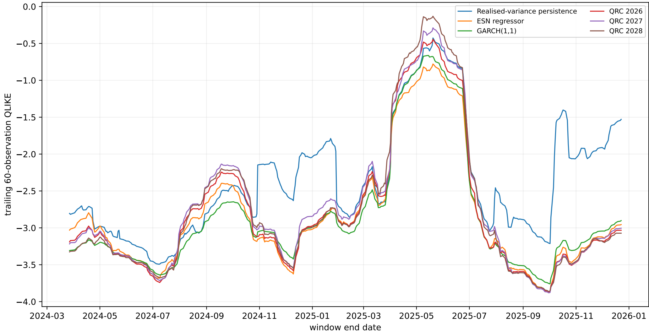
Descriptive rolling test QLIKE
