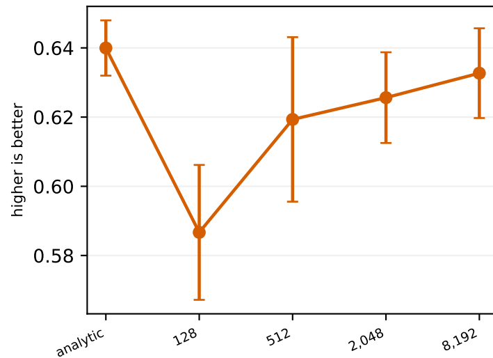
Transition PR-AUC
