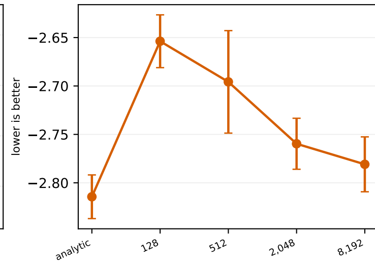
QLIKE
