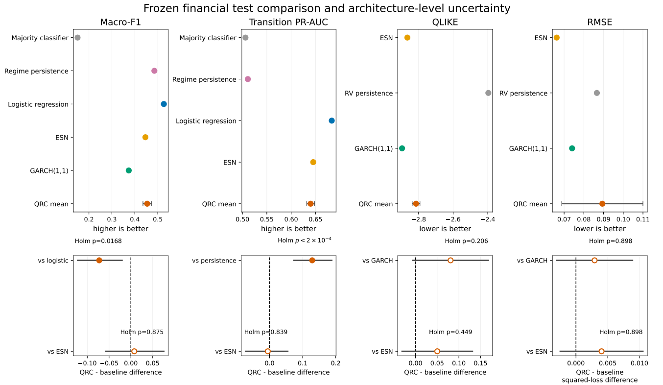
Figure 2: Frozen financial test estimates and selected architecture-level 95% intervals for QRC-minus-baseline differences. Filled markers denote Holm-adjusted support and hollow markers do not. QRC statistics average paired per-seed differences, not prediction ensembles. Logistic leads macro-F1, GARCH leads QLIKE and ESN leads RMSE. The persistence transition annotation uses the finite two-sided resolution of 10,000 strict empirical resamples rather than displaying p = 0 .
