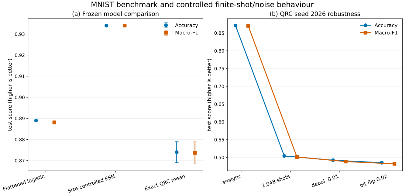
Figure 3: Genuine-MNIST test comparison and controlled robustness. Exact QRC bars show mean and population variation across three seeds; finite-shot/noise rows use frozen seed 2026. The 2,048-shot, depolarising and measurement-flip conditions are classical simulations, not hardware-calibrated experiments.
