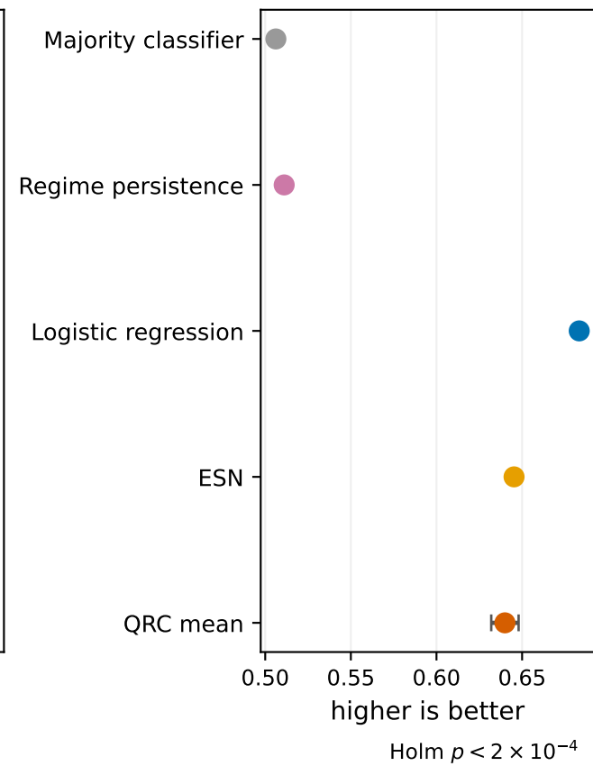
Transition PR-AUC
