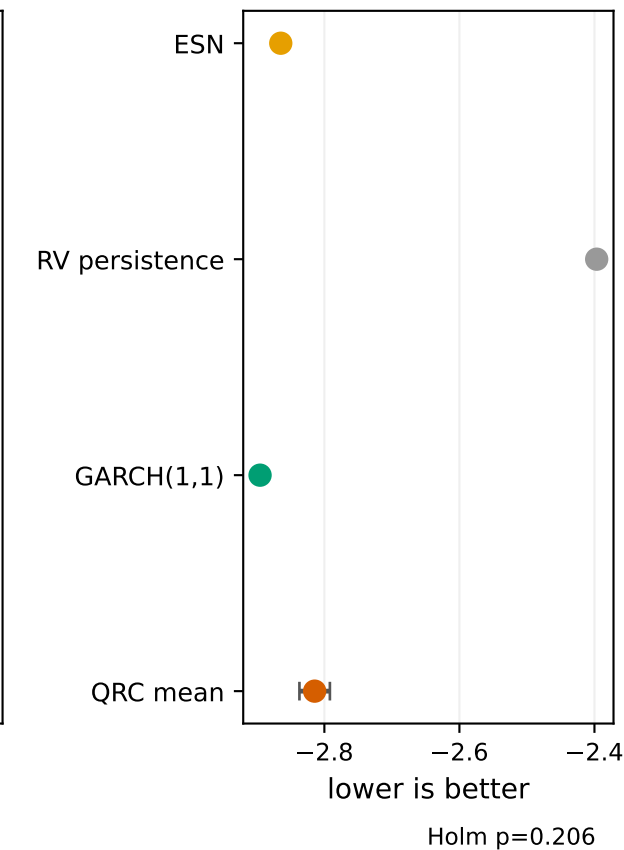
QLIKE
