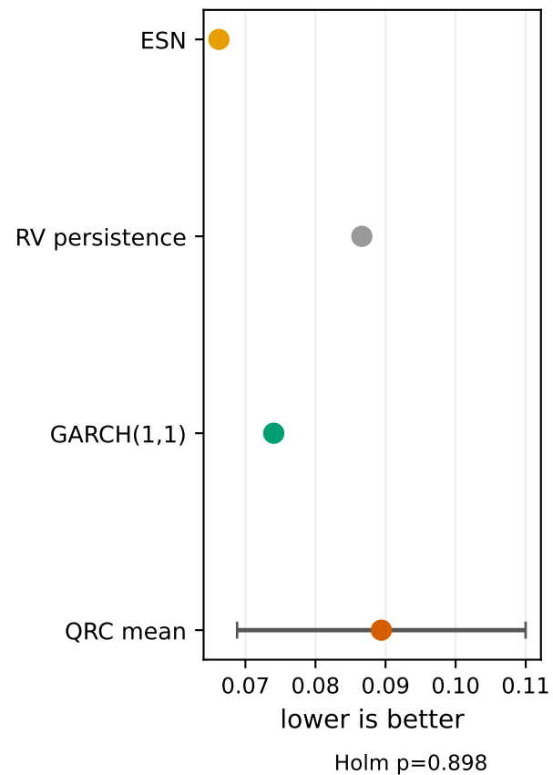
RMSE
