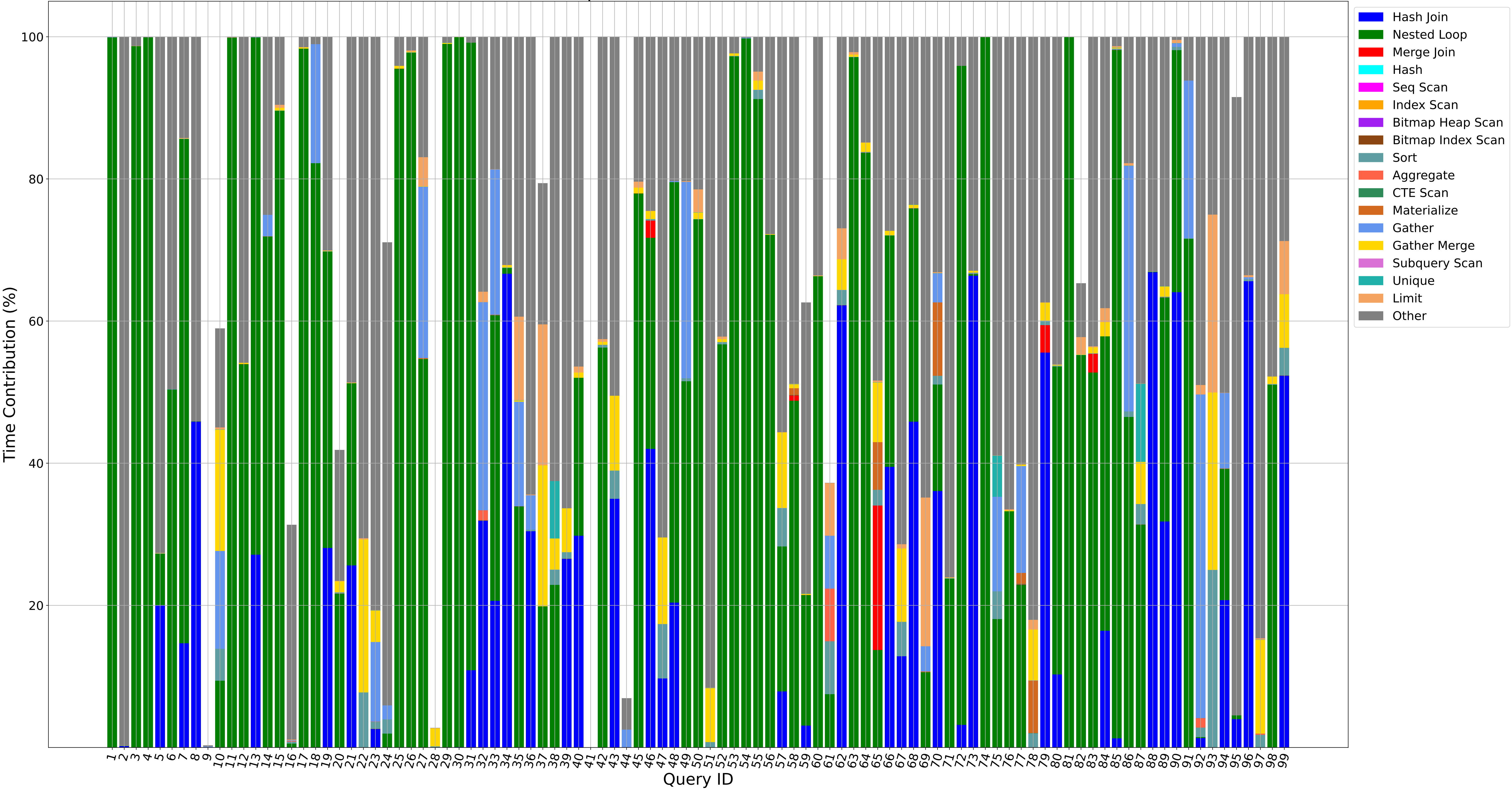
TPC-DS Operator Time Breakdown (Offline)
