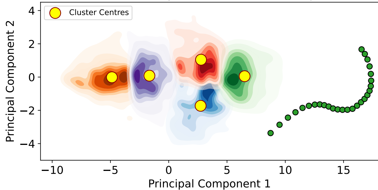
Cluster Density and Centres in PCA Space
