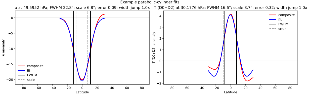
Figure 3: Parabolic-cylinder fits to zonal wind near 50 hPa and temperature near 30 hPa from ERA5. Solid and dashed markers show FWHM and fitted scale, respectively.
