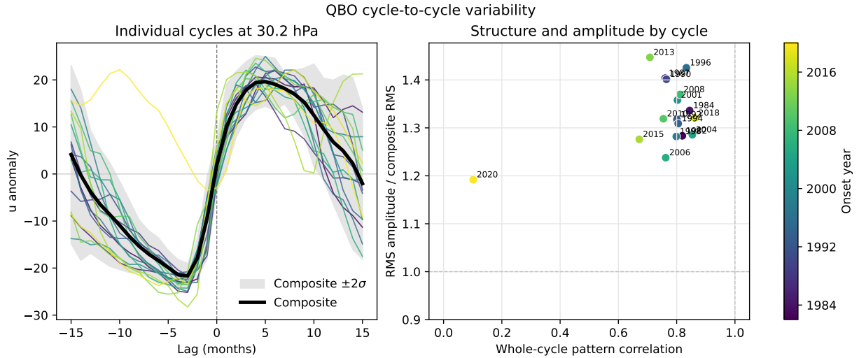
Figure 10: Westerly-onset QBO cycles at 30 hPa and their amplitude, timing and structure metrics from ERA5. The left panel shows the individual onset-aligned cycles (coloured by onset year), their composite (black), and the composite plus or minus two standard deviations across cycles (grey shading). The right panel shows whole-pattern correlation against RMS-amplitude ratio; colour and labels give onset year. Dashed lines mark zero lag in the left panel and unit correlation and amplitude ratio in the right panel. The standard deviation excludes pointwise values outside the standard 1.5-IQR limits.
