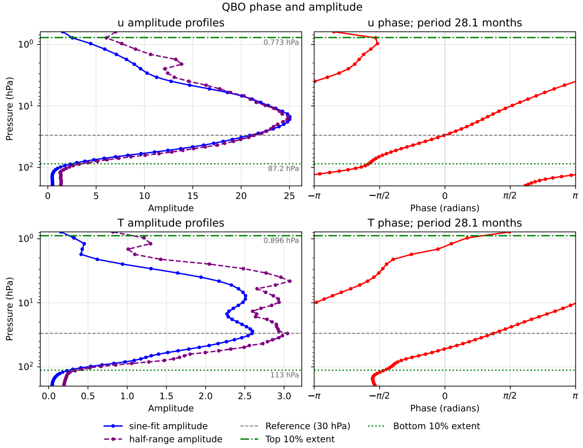
Figure 7: Amplitude and phase profiles for a QBO period of 28.05 months from ERA5. Blue solid lines show sine-fit amplitude. Purple dashed lines show half-range amplitude. Grey dashed and green dash-dot lines mark 30 hPa and the vertical extent, respectively.
