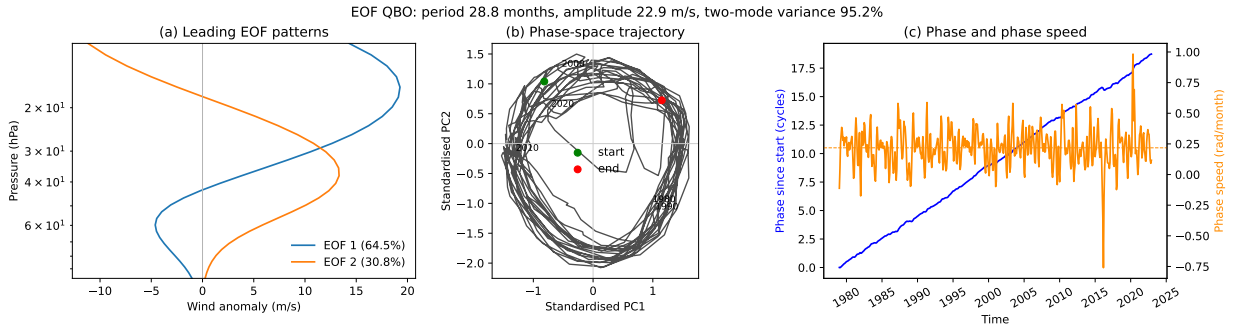
Figure 1: ERA5 leading EOF wind patterns, principal-component trajectory, phase, and phase speed for the full 1979–2022 monthly record. The wind is averaged over 5°S–5°N.
