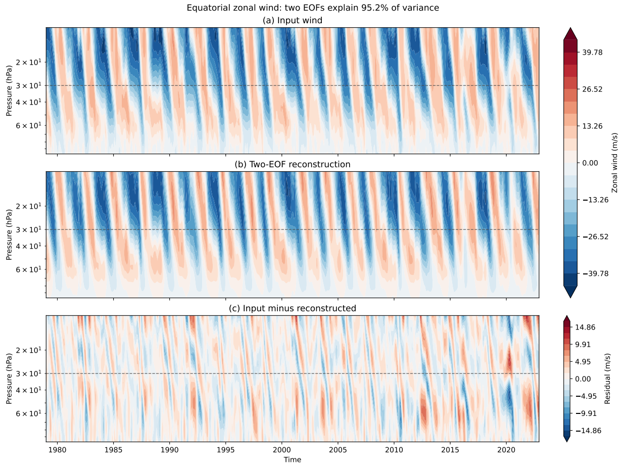
Figure 2: ERA5 zonal wind averaged over 5^{\circ}\text{S} – 5^{\circ}\text{N} , its two-EOF reconstruction, and the residual for 1979–2022. Both wind panels use the same colour scale.
