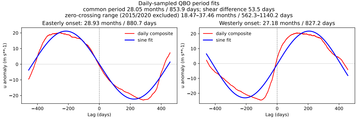
Figure 6: Daily ERA5 30-hPa composites and sine fits. The periods for different choices of onset differ by 53.5 days and average to 853.9 days (28.05 months). Individual zero-crossing periods range from 18.47 to 37.46 months. The calculation excludes the 2015 and 2020 onset years.
