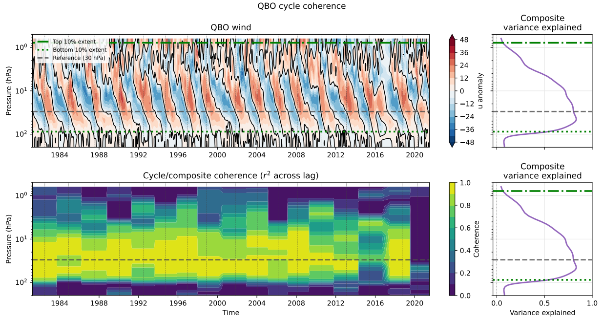
Figure 9: QBO-cycle anomalies, pressure-resolved coherence and composite variance explained. The variance profile repeats beside both pressure panels. The calculation includes the 2015 and 2020 onset years. Vertical dashed lines mark westerly onsets; the horizontal grey dashed line marks 30 hPa. Green dash-dot and dotted lines in the upper panel mark the top and bottom vertical extent, respectively.
