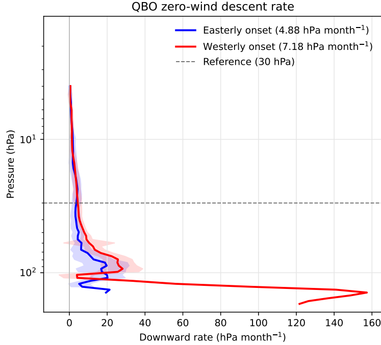
Figure 8: Pressure-resolved downward rates of the onset-connected zero-wind contours in the ERA5 easterly- and westerly-onset composites. Legend values are the mean monthly displacements. Shading spans one standard deviation across individual QBO cycles and the grey dashed line marks 30 hPa.
