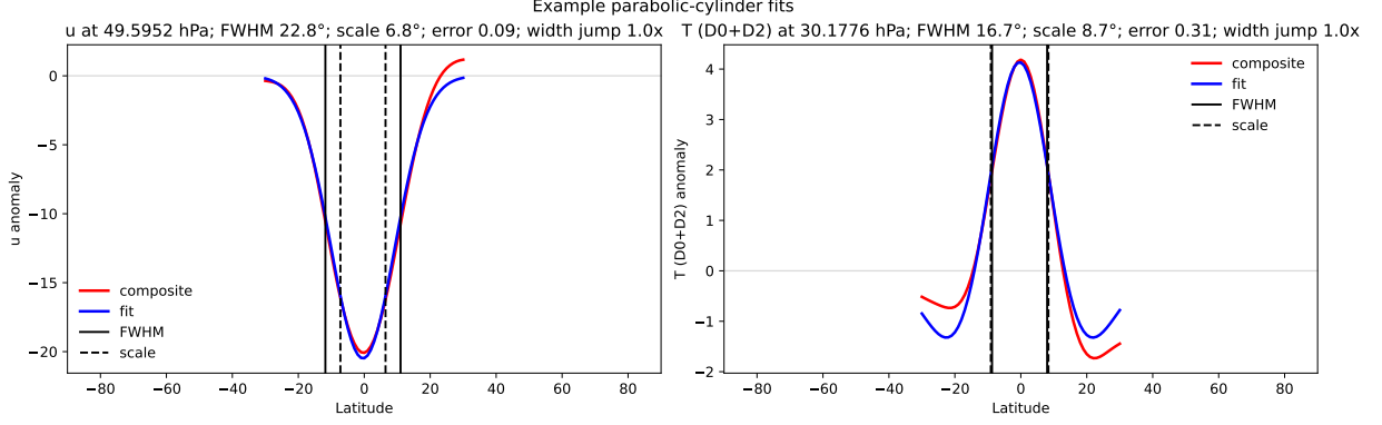
Figure 5: Parabolic-cylinder fits to zonal wind near 50 hPa and temperature near 30 hPa from ERA5. Solid and dashed markers show FWHM and fitted scale, respectively.
