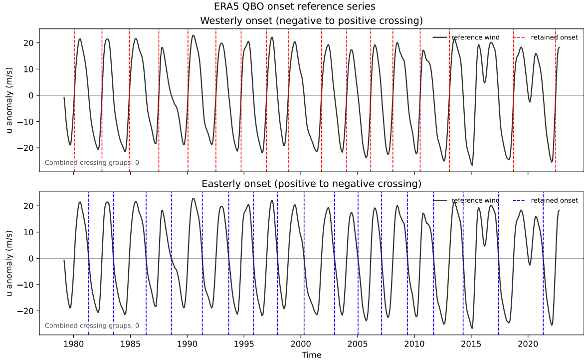
Figure 3: Monthly 30-hPa reference timeseries r(t) for westerly and easterly onsets from ERA5. Dashed lines mark zero crossings. A merged pair of nearby crossings would be shown by an orange interval and dotted original crossings; none occur in this dataset.
