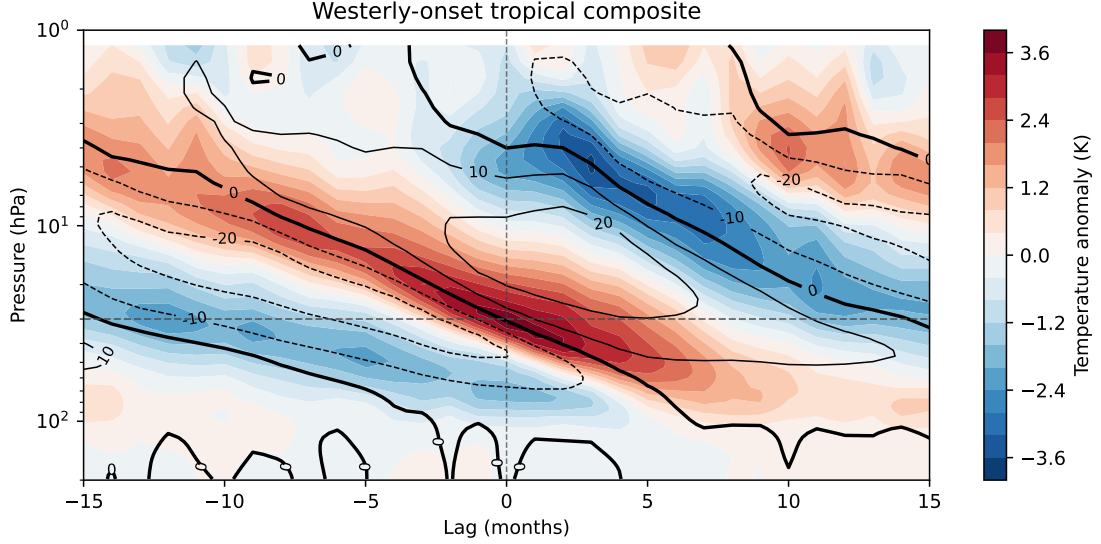
Figure 4: 5°S–5°N mean westerly-onset composites from ERA5. Filled contours are temperature anomalies (K); line contours are zonal-wind anomalies ( \text{m s}^{-1} ). The grey dashed line marks the 30-hPa reference pressure.
