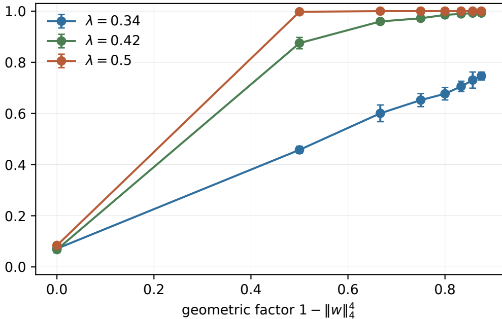
detection power
