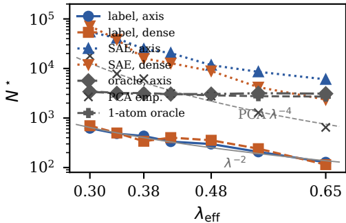
Labels vs free SAE N^*
