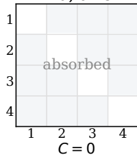
ind, axis
