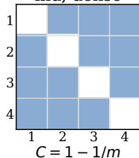
ind, dense
