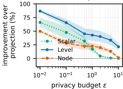
uniform signals
