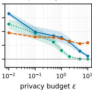
sparse signals
