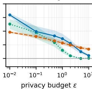
random signals
