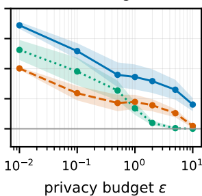
smooth signals
